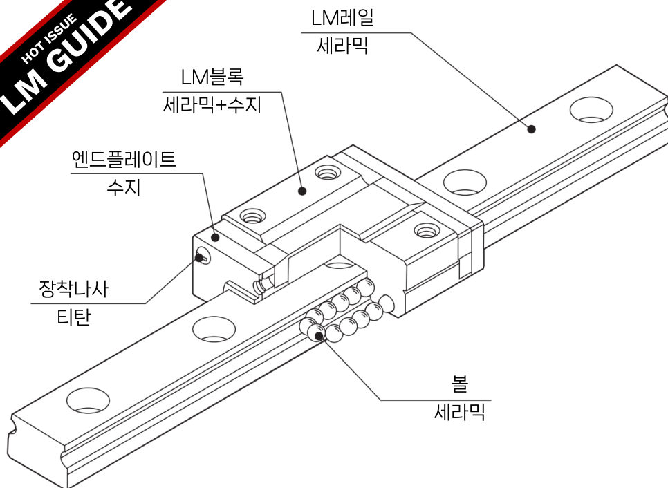
Ceramic LM Guide RSR-Z
